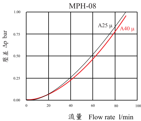
壓降曲線圖 Housing pressure drop curve
