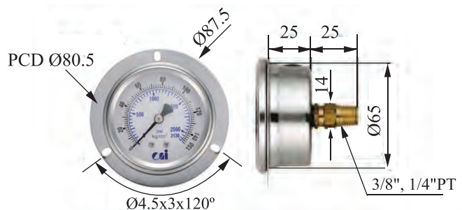
埋入式 CBM- 60 __ kg/psi* _ / _ " PT Mounting
