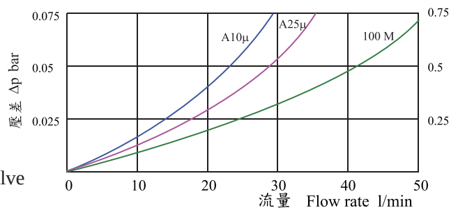
壓降曲線圖 Housing pressure drop curve
